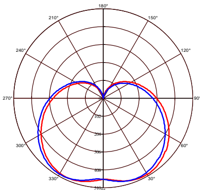
Photometric Diagram
