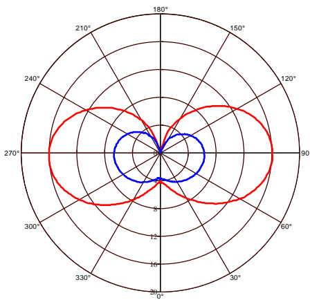
Photometric Diagram
