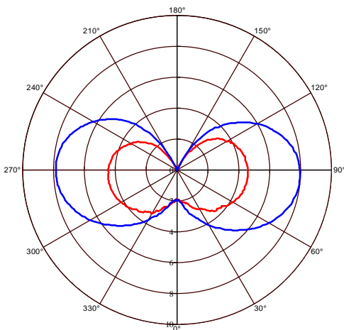
Photometric Diagram
