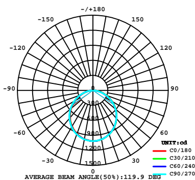
Photometric Diagram
